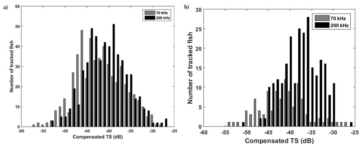
Figure 2.3. Mean target strength (TS) distribution (dB re 1 \text{ m}^2 ) of echoes attributed to (a) black and (b) ocean triggerfish at 200) and 70 kHz. Data are from the FAROFA2 survey.
