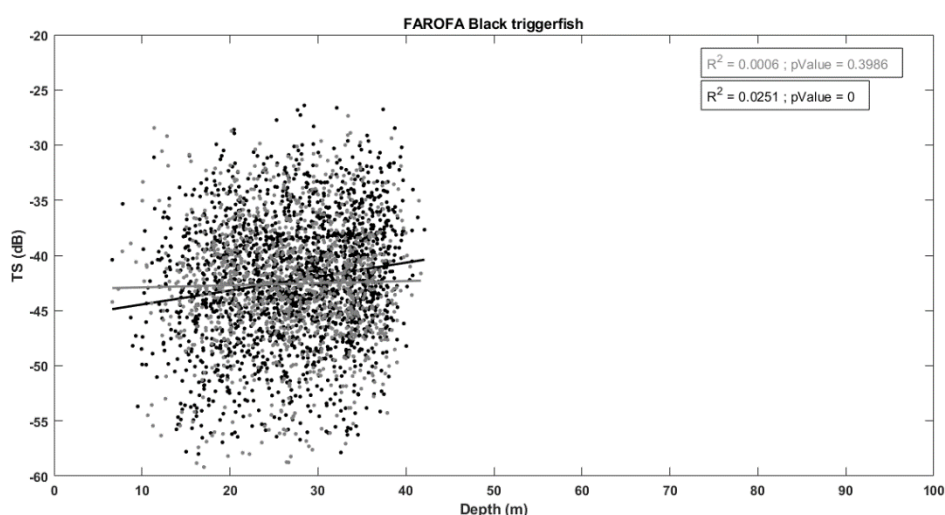
Supplementary Figure S2.1. Depth–TS diagram for black triggerfish in 70 kHz (grey) and 200 kHz (black).
