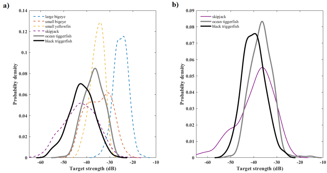
Figure 2.4. (a) Normalised density functions of target strength (TS) distribution (dB re 1 m 2 ) at 38 kHz for a 60-cm yellowfin tuna and 110-cm bigeye tuna from Bertrand et al. (1999); fish aggregating device (FAD)-aggregated tuna mix dominated by small (,50-cm) bigeye tuna Thunnus obesus (92%), Thunnus albacares (7%) and Katsuwonus pelamis (1%) from Josse and Bertrand (2000); tuna mix dominated by skipjack K. pelamis (99%) and T. albacares (1%) from Boyra et al. (2018); and at 70 kHz for black and ocean triggerfish from the FAROFA2 survey. TS distributions represented by dotted and solid lines were measured at a frequency of 38 and 70 kHz respectively. (b) Normalised density functions of TS distribution (dB re 1 m 2 ) at 200 kHz of a tuna mix dominated by skipjack K. pelamis (99%) and T. albacares (1%) from Boyra et al. (2018) and black and ocean triggerfish from the FAROFA2 survey.
