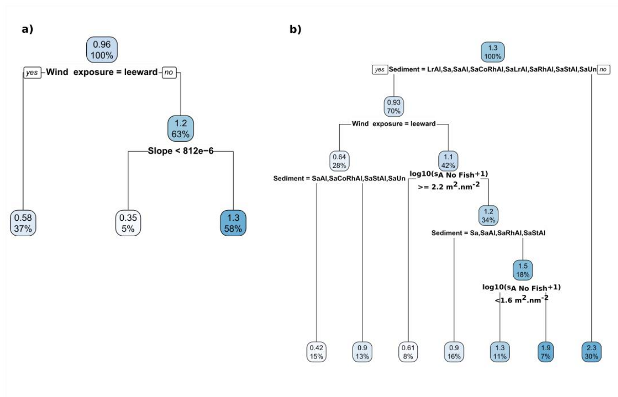
Figure 3.4. Regression tree on values of the fish-like acoustic biomass ( \log_{10}(s_A+1) ) performed on the complete data set (a) and the dataset limited to the locations where sediment was observed (b). The values inside each leaf is the mean fish-like acoustic biomass ( \log_{10}(s_A+1) ) and the corresponding percentage of ESDU.
