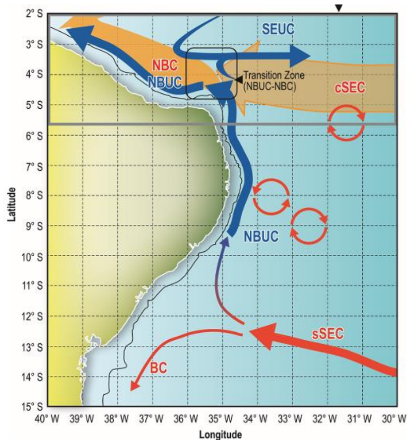
Figure 1.3. Schematic representation of mean currents and eddy generation along the Northeast Brazilian coast from Dossa et al., 2021
