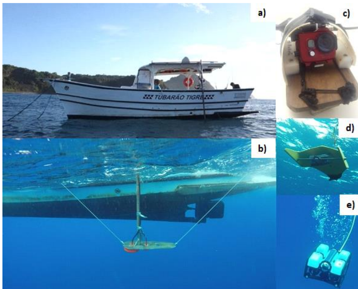
Supplementary Figure S3.1. Setting up of operations a) sport fishing boat “Tubarão tigre”; b) acoustic transducers (70 and 200 kHz) attached on a pole; c) vertical video system; d) towed video; e) ROV. Images were obtained by the authors.
